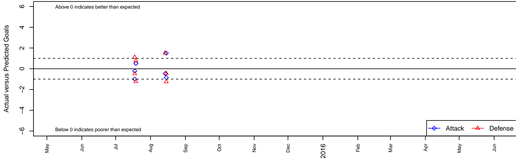
FPSC Mighty Dragons B02 Dots are actual minus expected GF (blue circles) and GA (red triangles). Blue line is smoothed change in attack strength. Red is smoothed change in defense strength.
